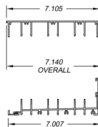
3-Track Frame Depth For Box Riser add .590"
