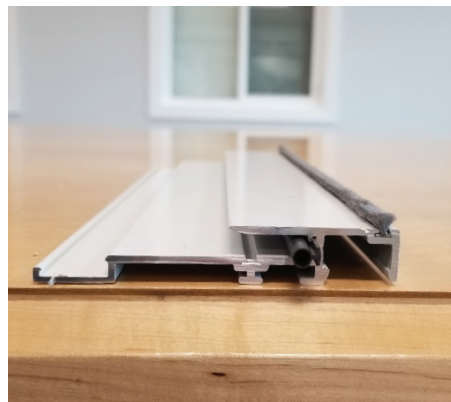
P-hook narrow riser (ordered by unit size or actual cut size)
