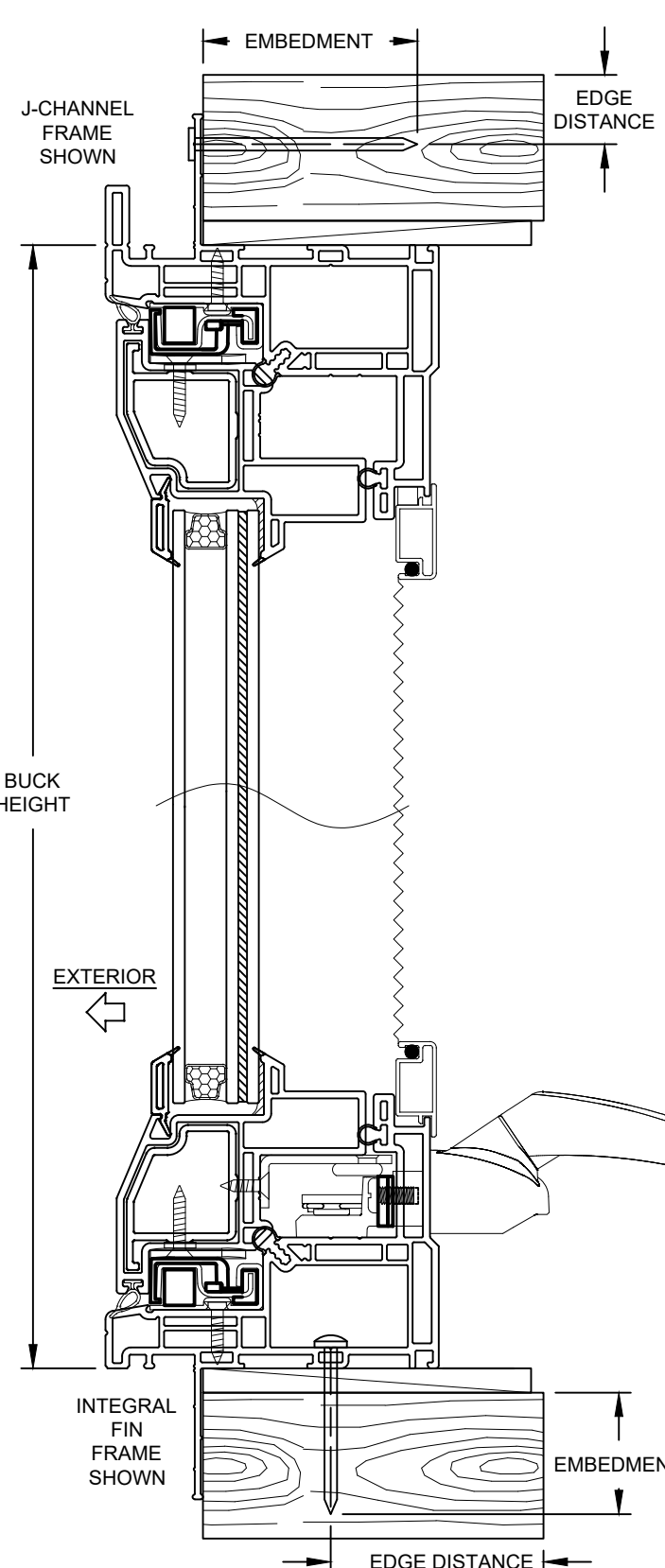
VERTICAL SECTION D-D SHOWN WITH HEAVY-DUTY SASH, HARDWARE & REINFORCEMENT
