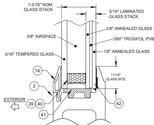
GLASS TYPE 4 USED IN DOOR
