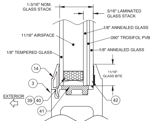
GLASS TYPE 3 USED IN DOOR
