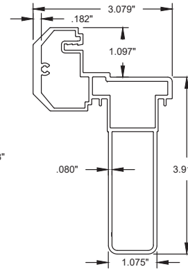
9 INACTIVE ASTRAGAL #20017, 6063-T6
