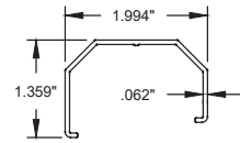
13 INACTIVE ASTRAGAL COVER #20004, Rigid PVC
