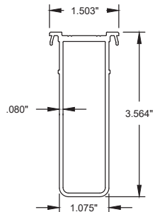
5 HINGE STILE REINFORCEMENT #20013, 6063-T6
