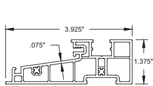
2 FRAME SILL #20001, Rigid PVC
