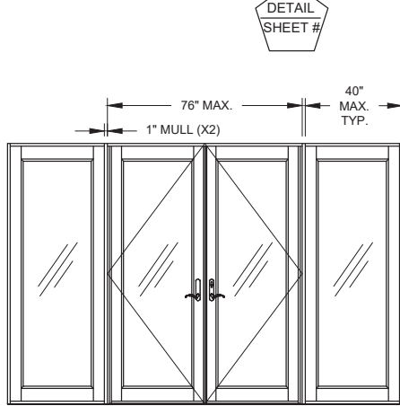
O/XX/O (WIDE STILES AND WIDE RAILS SHOWN ON SIDELITES)
