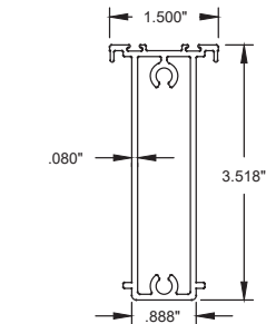
6 TOP & BOTTOM RAIL REINFORCEMENT #20014, 6063-T6
