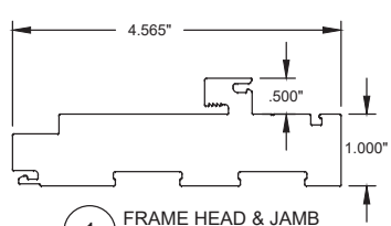
1 FRAME HEAD & JAMB #20000, Cellular PVC
