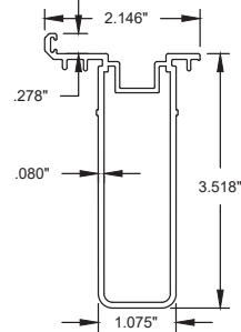
7 PANEL STILE REINFORCEMENT #20015, 6063-T6
