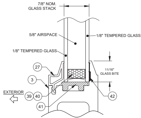
GLASS TYPE 1 USED IN DOOR, SIDELITE, TRANSOM
