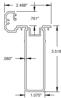
8 ACTIVE ASTRAGAL #20016, 6063-T6
