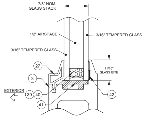
GLASS TYPE 2 USED IN DOOR, SIDELITE, TRANSOM
