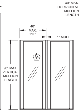
O/O (ADDITIONAL MULLED LITES ALLOWED) (WIDE STILES AND NARROW RAILS SHOWN ON SIDELITES)
