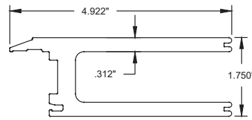
3 PANEL RAIL & STILE #20002, Cellular PVC
