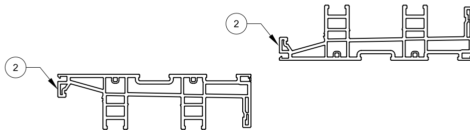
DETAIL H2 90° OUTSIDE CORNER
